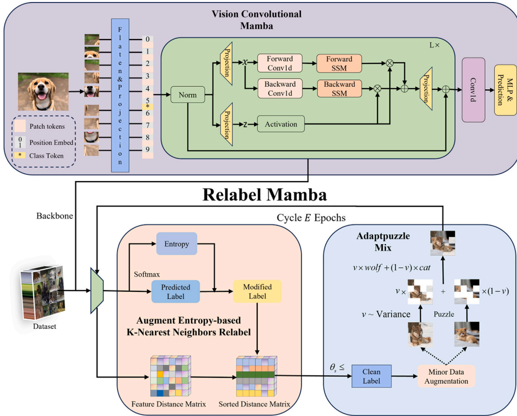
Fig. 2. Overview of our proposed RelabelMamba, which includes: Vcm to address the warm-up phase during pre-training; AEKR for noisy label correction, selection, and data augmentation; and the AdaptPuzzle method for utilizing soft labels.
