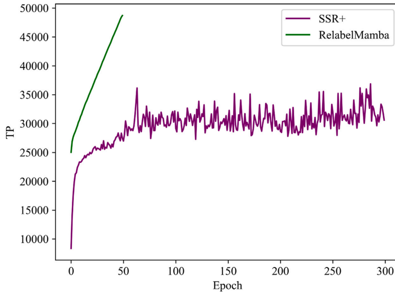
Fig. 4. Comparative analysis of label refine performance between RelabelMamba over 50 epochs and SSR+ over 300 epochs.
