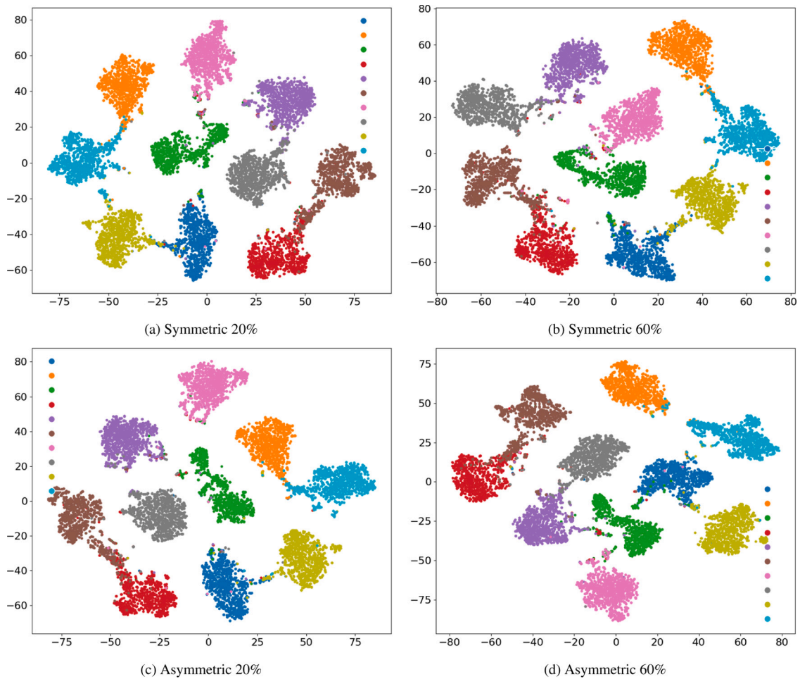
Fig. 5. The T-SNE visualizations provide insights into the network features of test images from the CIFAR-10 dataset, depicting the class distribution after 50 epochs of training with various noise types: symmetric at 20% and 60%, and asymmetric at 20% and 60%. Despite the challenges of extreme label noise, RelabelMamba's capability is evident in its effective learning of true class distributions. Each of the ten classes—Airplane, Automobile, Bird, Cat, Deer, Dog, Frog, Horse, Ship, Truck—is distinctly represented by a unique color: deep blue, vibrant orange, grassy green, bold red, muted purple, earthy brown, soft pink, medium gray, bright lime green, and clear aqua, respectively.
