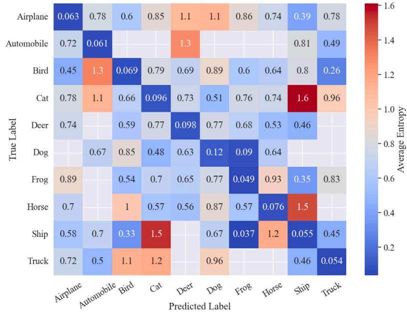
Fig. 1. Heatmap comparing the average entropy values between predicted and true labels. Darker shades of red indicate higher entropy values. The x-axis shows the predicted categories, while the y-axis represents the true categories.
