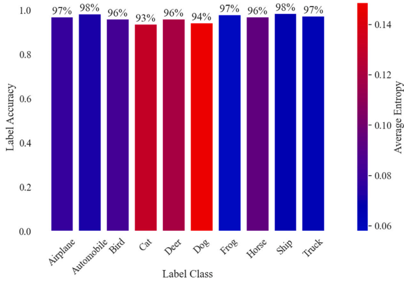
Fig. 3. The chart shows label rectification accuracy by class, with darker blue bars indicating higher model certainty and lower entropy.
